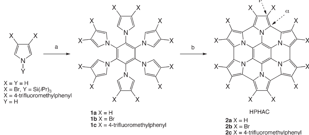
Scheme 1. Synthesis of annularly fused hexapyrrolohexaazacoronenes 2 (HPHAC). Reagents and conditions: a) NaH or NaOMe, DMF; then hexafluorobenzene; b) FeCl 3 , CH 3 NO 2 /CH 2 Cl 2 ; then hydrazine.
